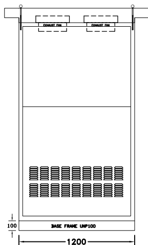
TAMPAK SAMPING
